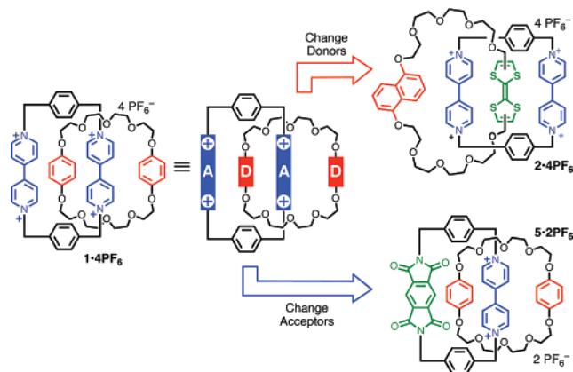
Scheme 1. Introducing Translational Isomerism by Varying the Donors or Acceptors in the [2]Catenane 1 ·4PF 6
